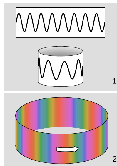
a / 1. Eight wavelengths fit around this circle ( \ell = 8 ). This is a standing wave. 2. A traveling wave with \ell = 8 , depicted according to the color conventions defined in figure u, p. 884.
